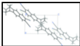
Fig. 2. A section of the crystal packing of the title compound, viewed down the b axis. Green dashed lines denote the intermolecular C—H...N hydrogen bonds.
